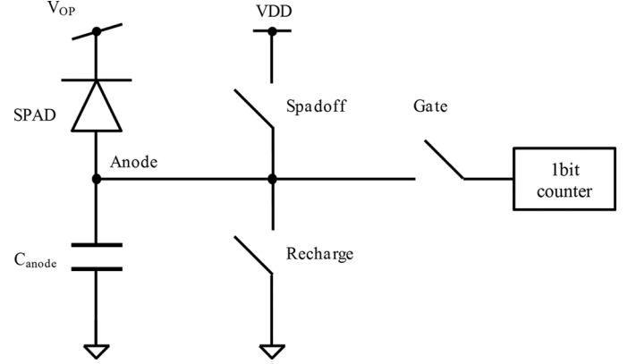
Fig. 1. Conceptual view of a gated SPAD.
