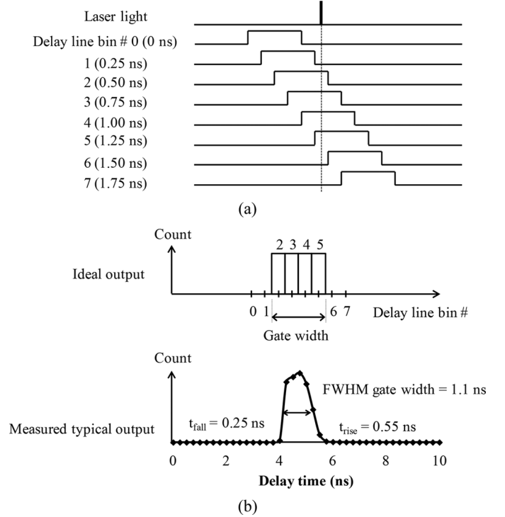
Fig. 9. (a) Gate-width measurement scheme. (b) Measured 1.1-ns gate width with rise and fall time.
