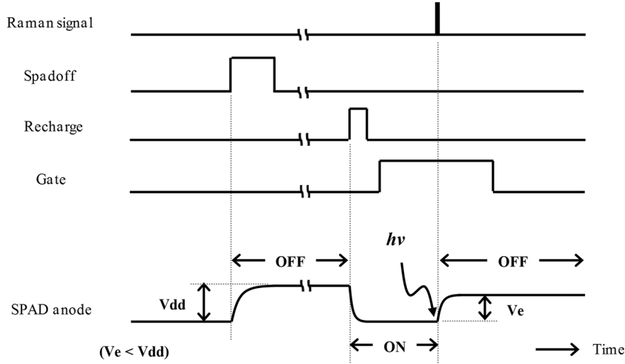
Fig. 3. Timing diagram of the gated operation.
